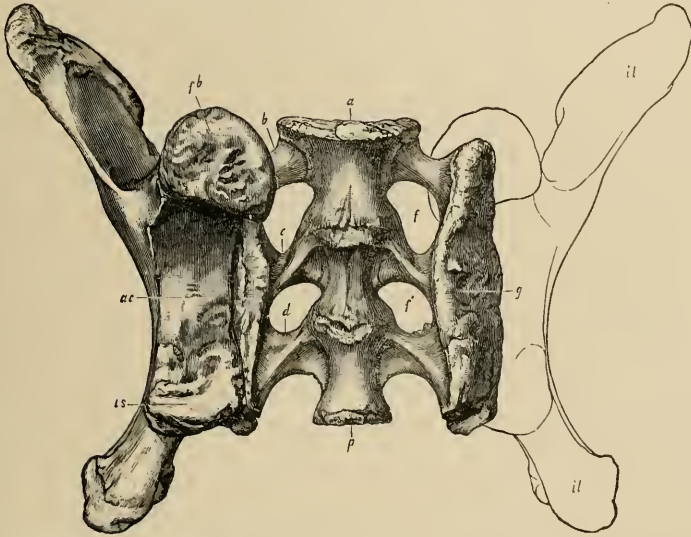
FIG. 10. Sacrum and ilium of Diplodocus longus Marsh; seen from below. With anterior and posterior ends of sacrum reversed. pb , pubic process; is , ischia process; ac , acetabulum; b , c , d , sacral ribs; f , f' , foramina. One tenth natural size. After Marsh.
