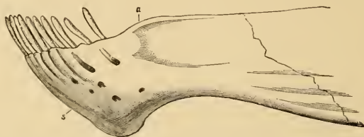
FIG. 2. Dentary bone of Diplodocus longus , seen from the left. One third natural size. a , edentulous border; s , symphysis. After Marsh.
